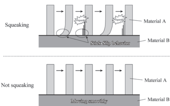
Fig.1 The image of squeaking mechanism
