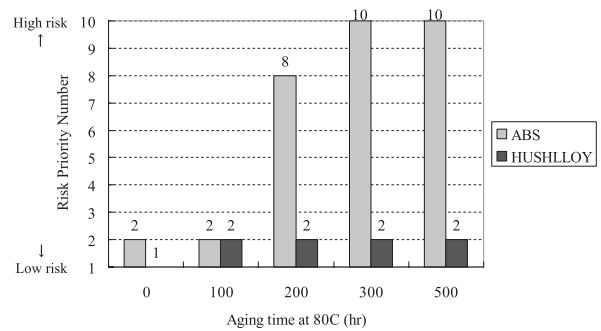
Fig. 7 Effect of thermal aging for squeak risk
