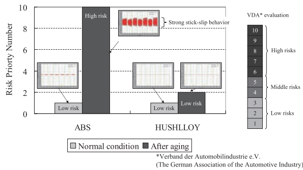
Fig. 6 The results for squeak risks from stick-slip tester
