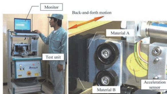
Fig.5 Stick-slip tester (Ziegler GmbH, stick-slip tester SSP-02)
