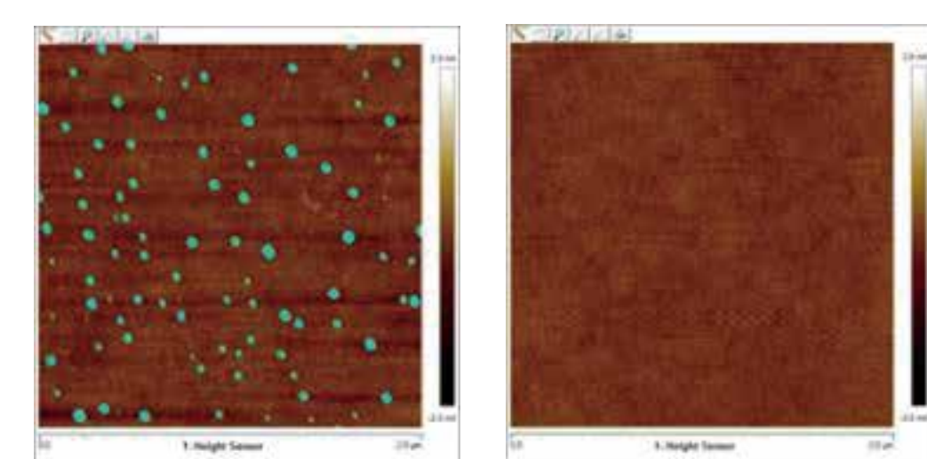
Surface roughness of PE-SiN
